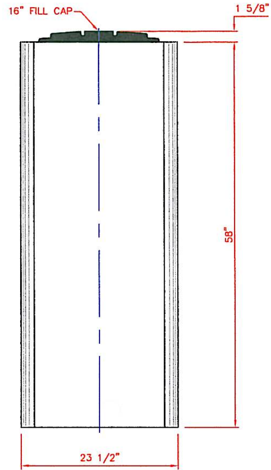
VIEW A
