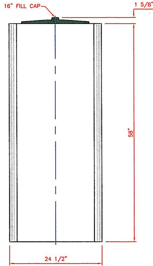
VIEW B
