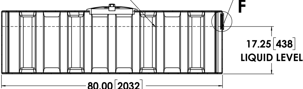
SECTION E-E SCALE 1 : 20
