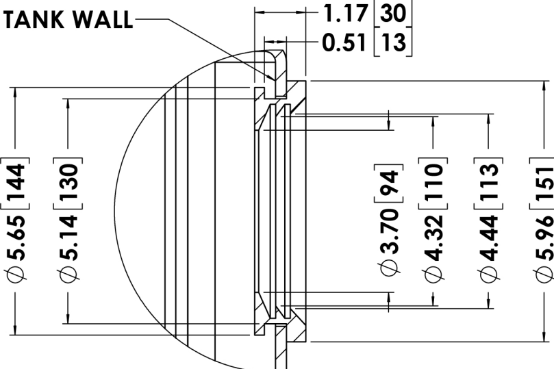
DETAIL F INLET FITTING 4" GROMMET SCALE 1 : 3
