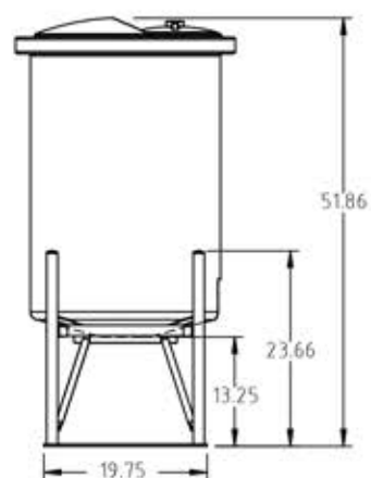
CB023-15ST METAL STAND
