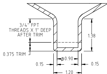
SECTION B-B SCALE 1:2
