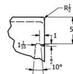
DETAIL A SCALE 0.12 : 1
