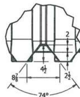
DETAIL A SCALE 1 / 11
