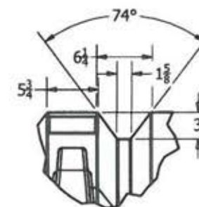
DETAIL B SCALE 1 / 11
