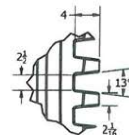
DETAIL C SCALE 1 / 11
