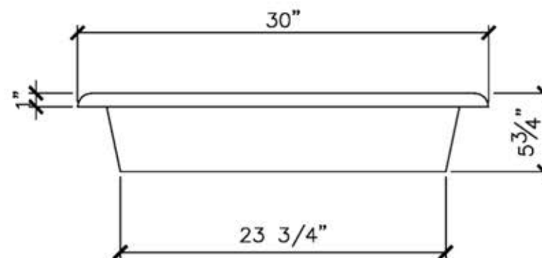
VIEW B
