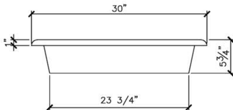
VIEW A
