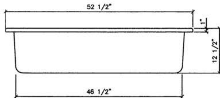
VIEW A
