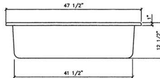
VIEW B
